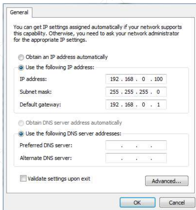
Figure 4-1 Internet Protocol Version 4 (TCP/IPv4)
